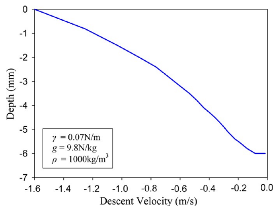
Figure 6. Variation of the descent velocity as the microrobot falls on the water surface.
